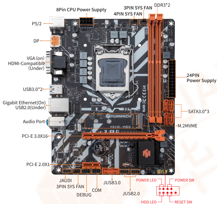
1-1 H310C-VHD3 motherboard illustration
