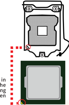
Figure 2-6 CPU installation
